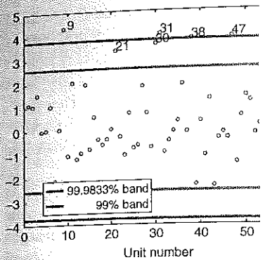
Fig. 2 Index plots of robust scale residuals based on a 50% breakdown point. The left-hand panel: 99% nominal efficiency and simultaneous bands using the standard
