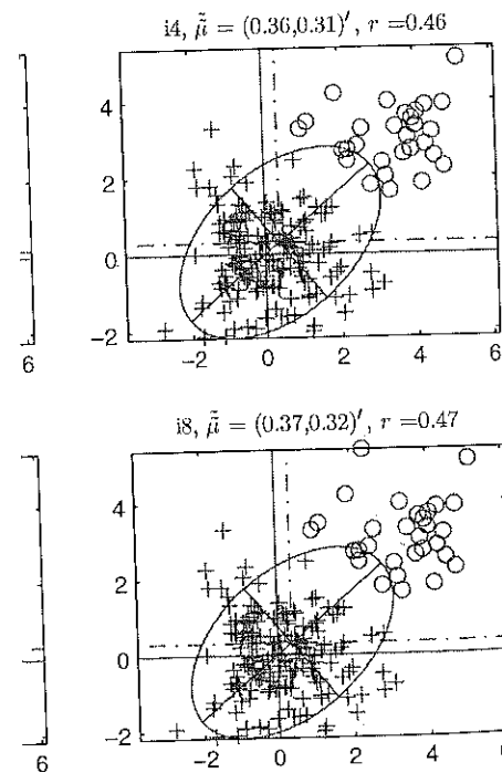
ability contours at different iterations of the algorithm, for a data set simulated from the contamination and \lambda = 3
