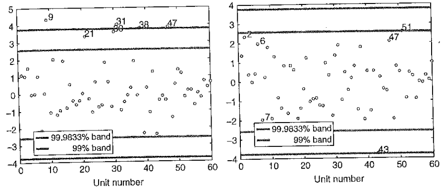
Fig. 2 Index plots of robust scale residuals obtained using MM estimation with a preliminary S -estimate of scale based on a 50% breakdown point. Left-hand panel: 90% nominal efficiency; right-hand panel: 95% nominal efficiency. The horizontal lines correspond to the 99% individual and simultaneous bands using the standard normal
